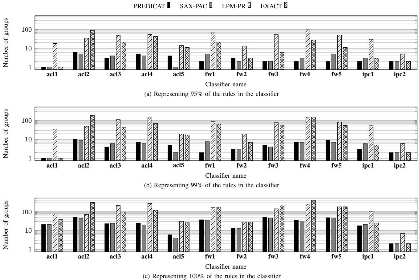
Fig. 2: Number of groups needed by each of the evaluated approaches to represent a fixed fraction – 95%, 99%, or 100% – of the classifier rules when the filter width is unrestricted, i.e., at the maximum of 104 characters.
