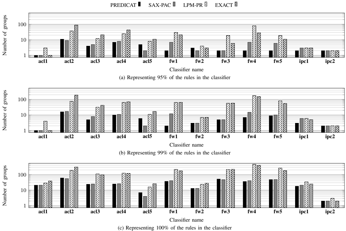
Fig. 1: Number of groups needed by each of the evaluated approaches to represent a fixed fraction – 95%, 99%, or 100% – of the classifier rules when the filter width is restricted to 32 characters for PREDICAT, LPM-PR and SAX-PAC.
